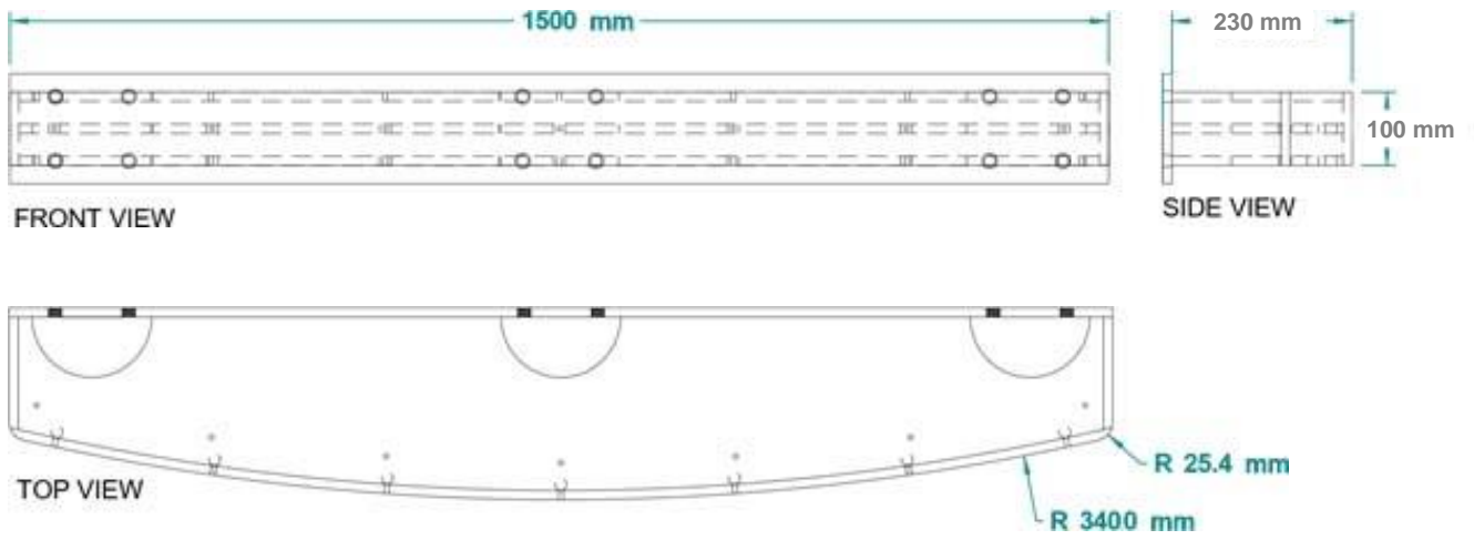
Figure 13: Main Barrier Dimensions, top view
