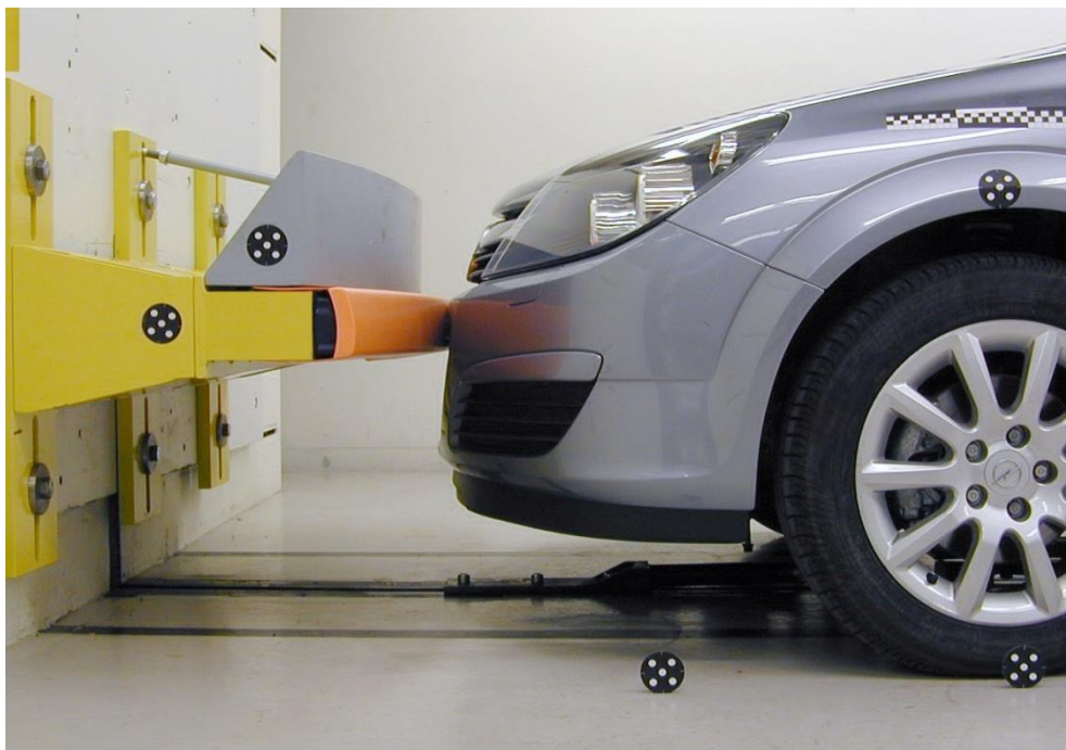
Figure 1: Bumper Barrier
