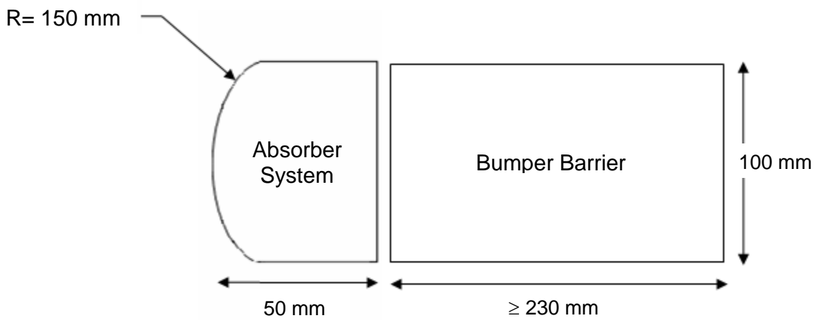
Figure 9: Bumper Barrier and Energy Absorber, Section A-A
