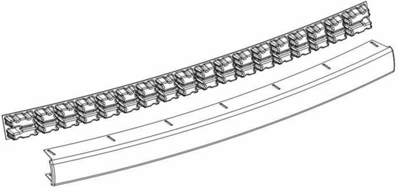
Figure 10: Energy Absorber and Bumper Cover
